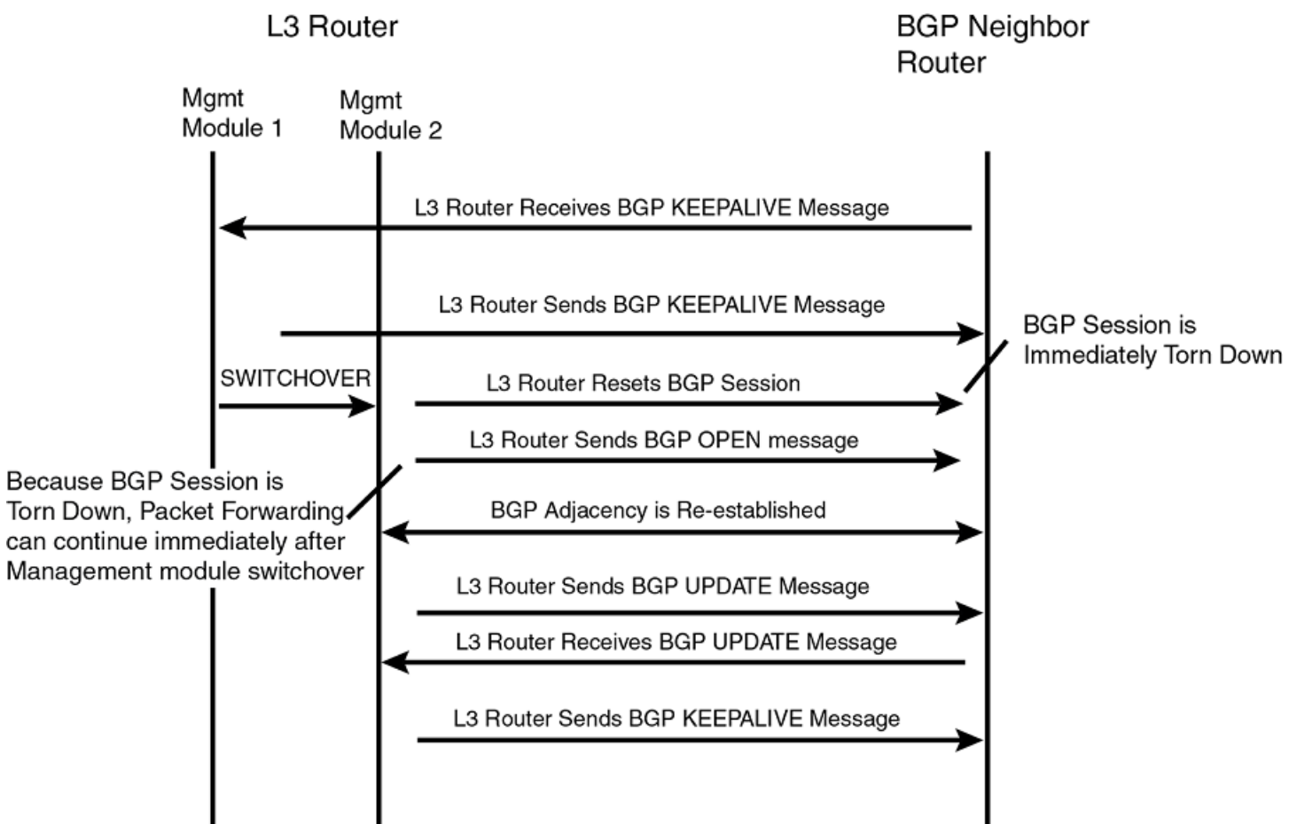
FIGURE 30 Management module switchover behavior for BGP4 peer notification
