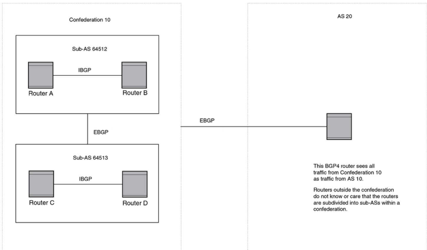
FIGURE 34 Example BGP4 confederation
