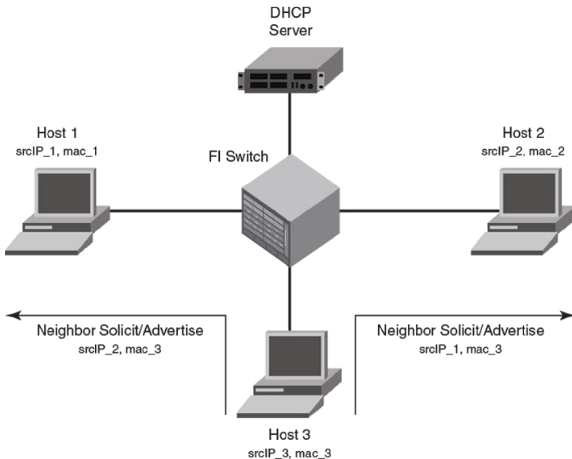
FIGURE 12 Neighbor discovery cache poisoning
