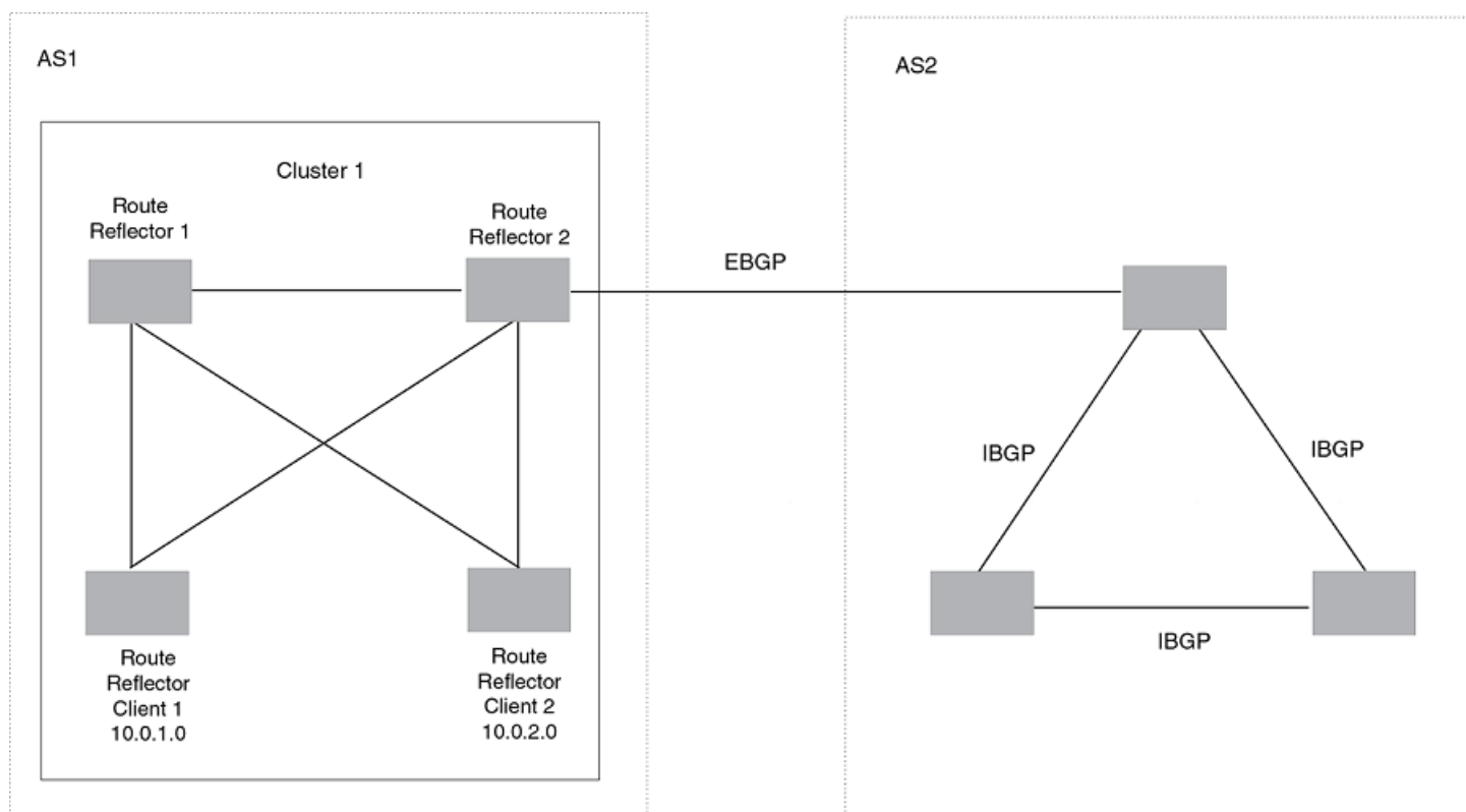
FIGURE 33 A route reflector configuration
