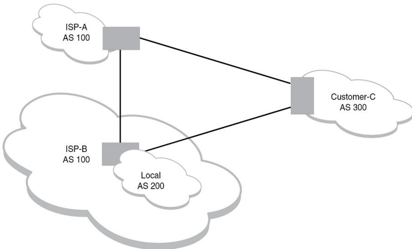
FIGURE 32 Example of Local AS configured on ISP-B
