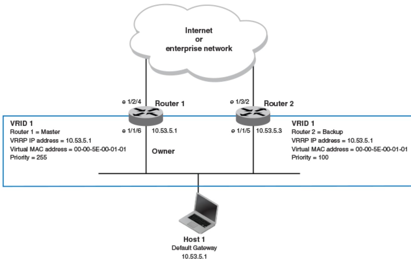
FIGURE 38 Basic VRRP topology
