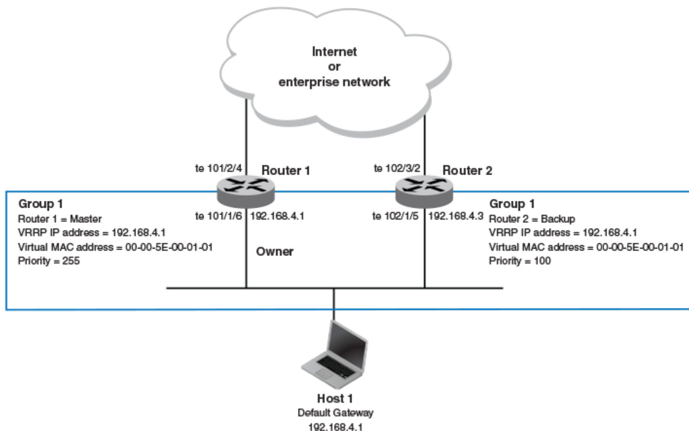
FIGURE 37 Devices configured as VRRP virtual routers for redundant network access for Host 1
