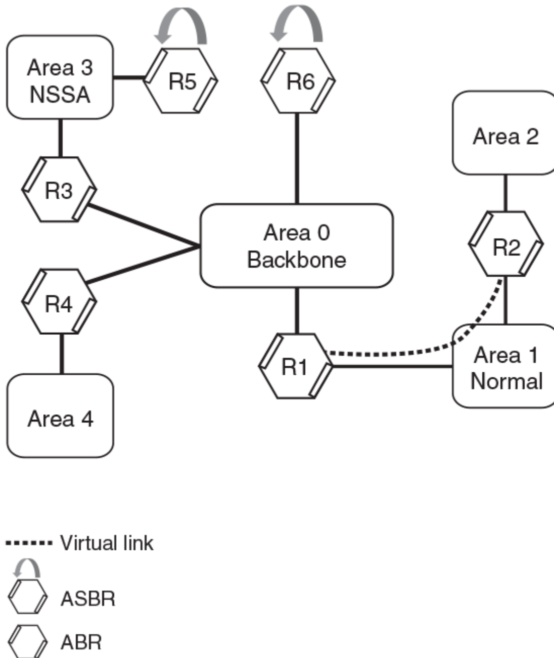
FIGURE 28 OSPFv3 virtual link
