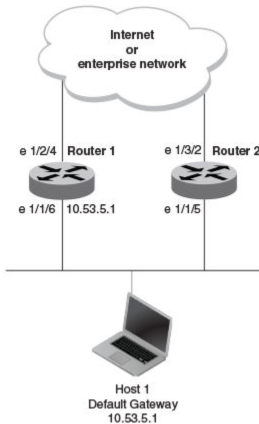
FIGURE 36 Single point of failure with Device 1 being the Host1 default gateway
