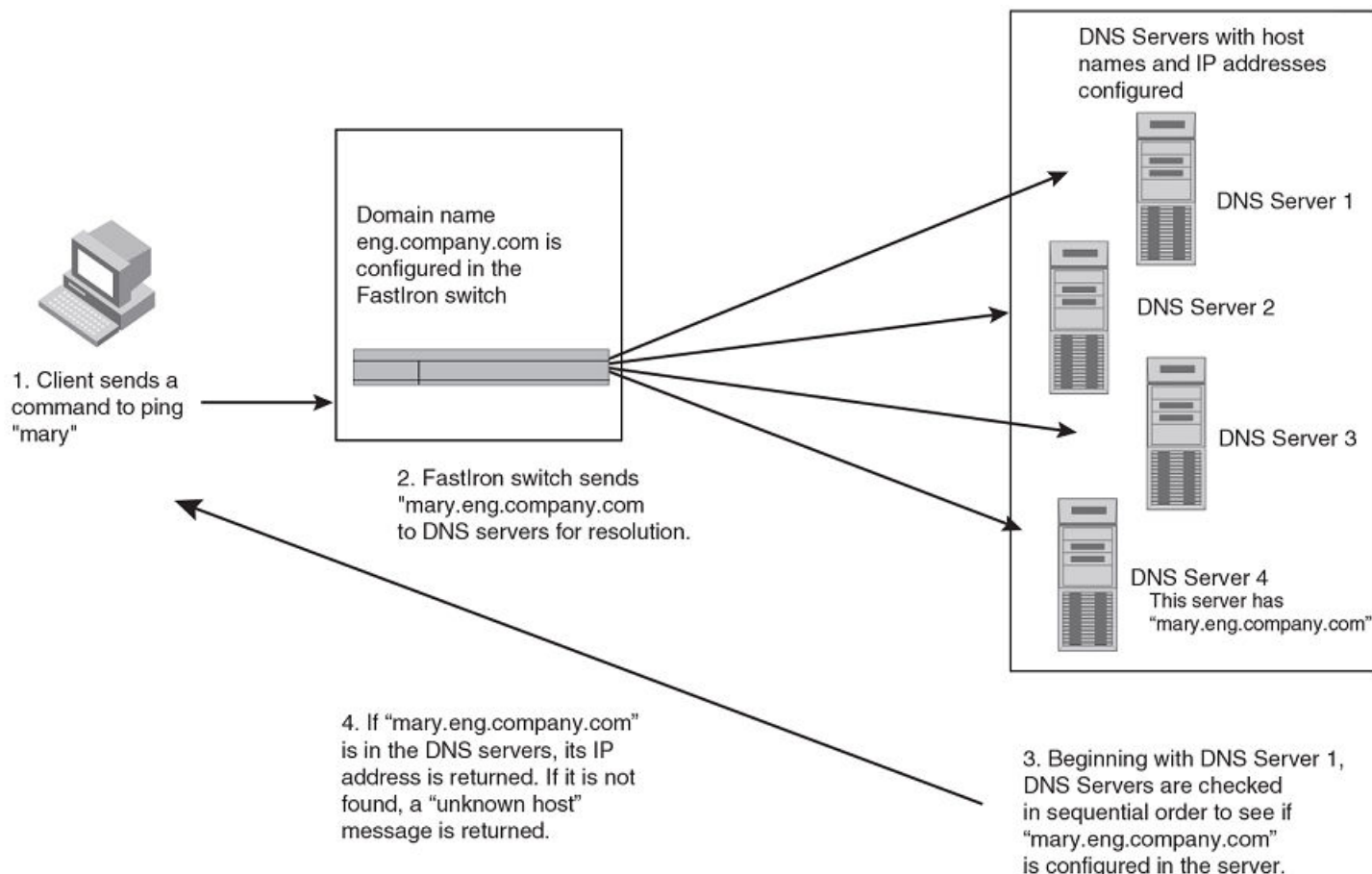
FIGURE 5 DNS resolution with one domain name
