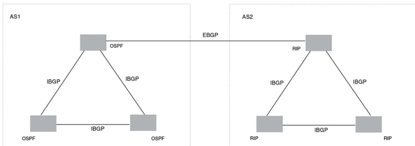
FIGURE 31 Example of customer connected to two ISPs
