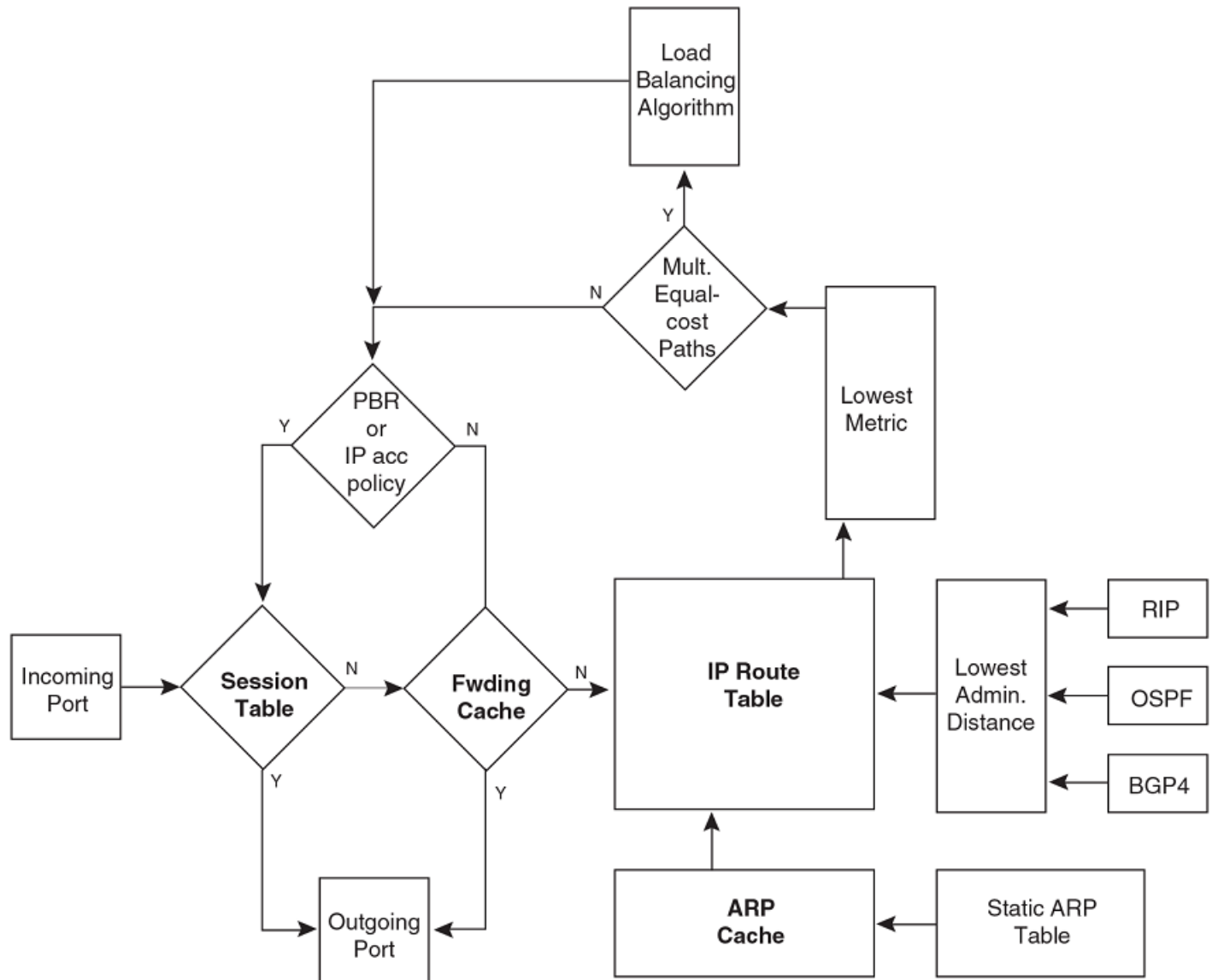
FIGURE 3 IP Packet flow through a Brocade Layer 3 switch
